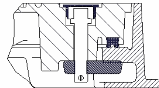
Detail: Locking System
